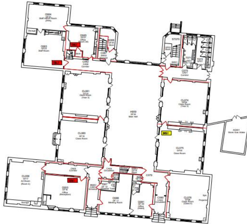
Junior School - Ground Floor Plan
